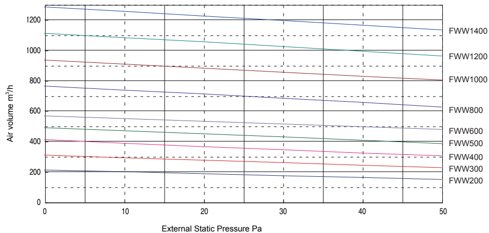
External Static Pressure 30Pa L speed
